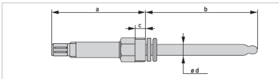
Figure 7-1: SMARTPAT ORP 8150
