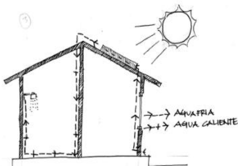
Figura 27. Panel solar individual
