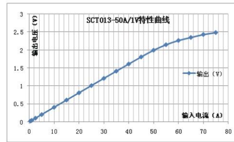
Characteristic curve in different load volt-ampere:
