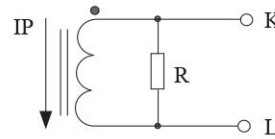
Built-in with sampling resistance voltage output type
